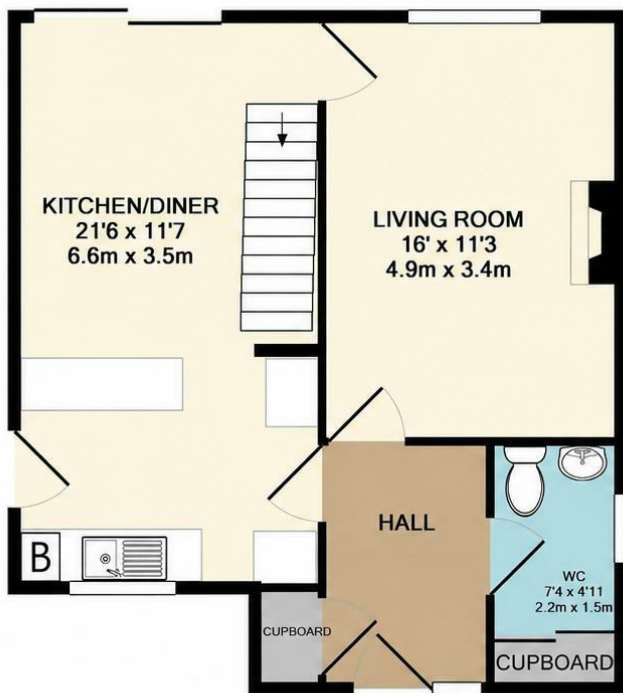
GROUND FLOOR APPROX. FLOOR AREA 50.5 SQ.M. (544 SQ.FT.)
